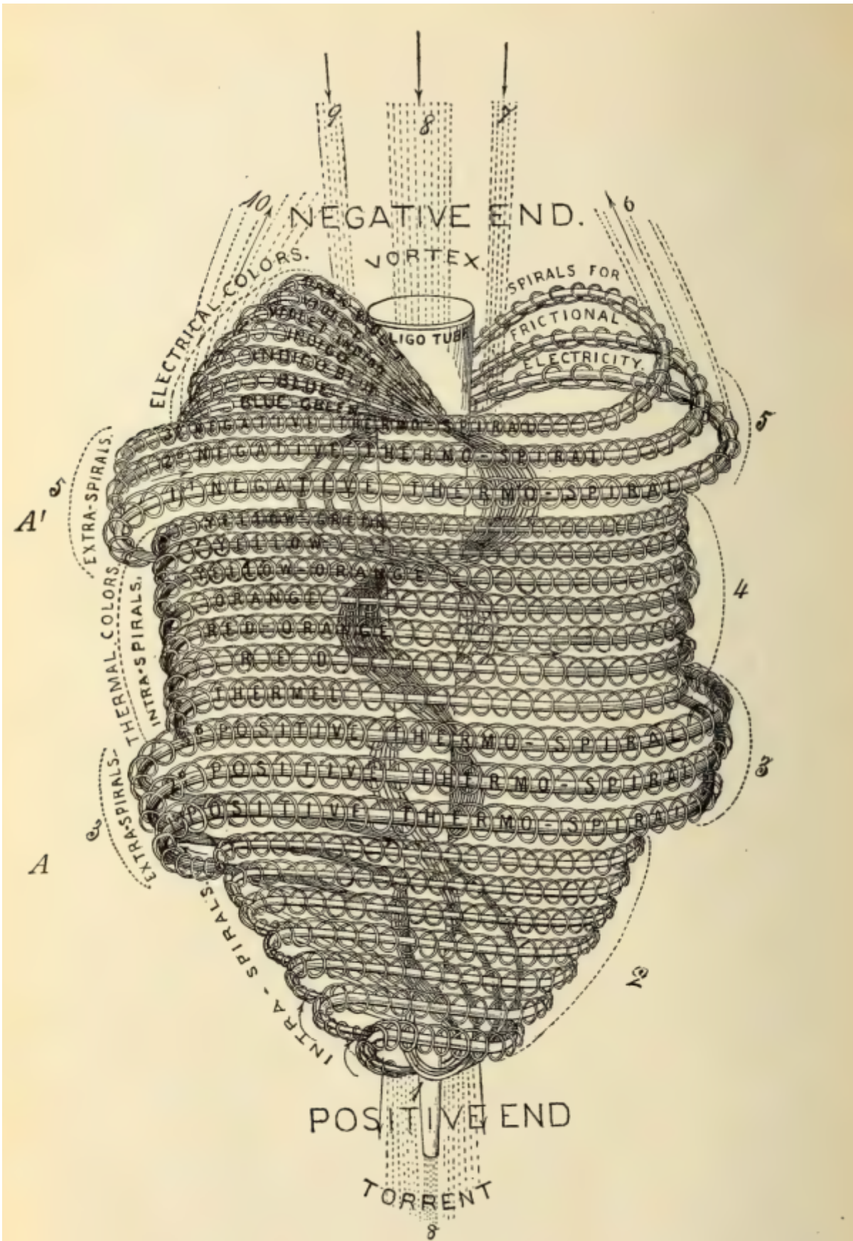
Fig. 135. The general Form of an Atom, including the spirals and 1st Spirillæ, together with influx and efflux ethers, represented by dots, which pass through these spirillæ. The 2d and 3d spirillæ with their still finer ethers are not shown.
